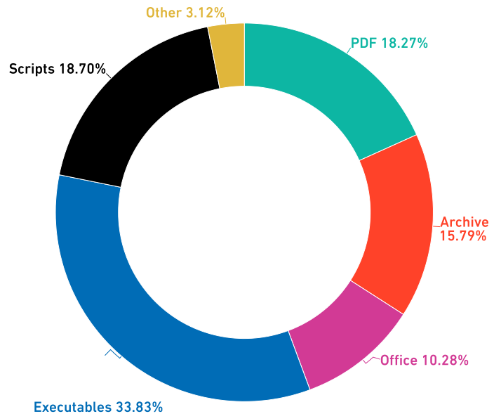
2022 New Malicious File Type Detections | Capture ATP
