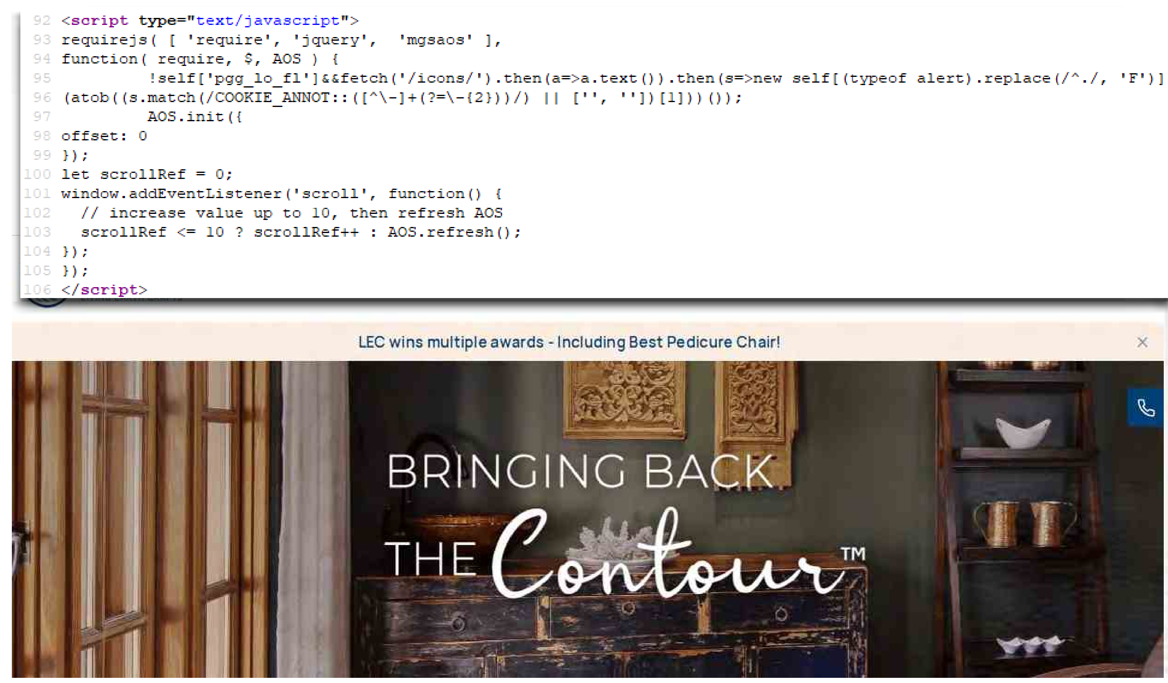
Website compromised by JS/Spy.Banker and the malicious code linked to the page
