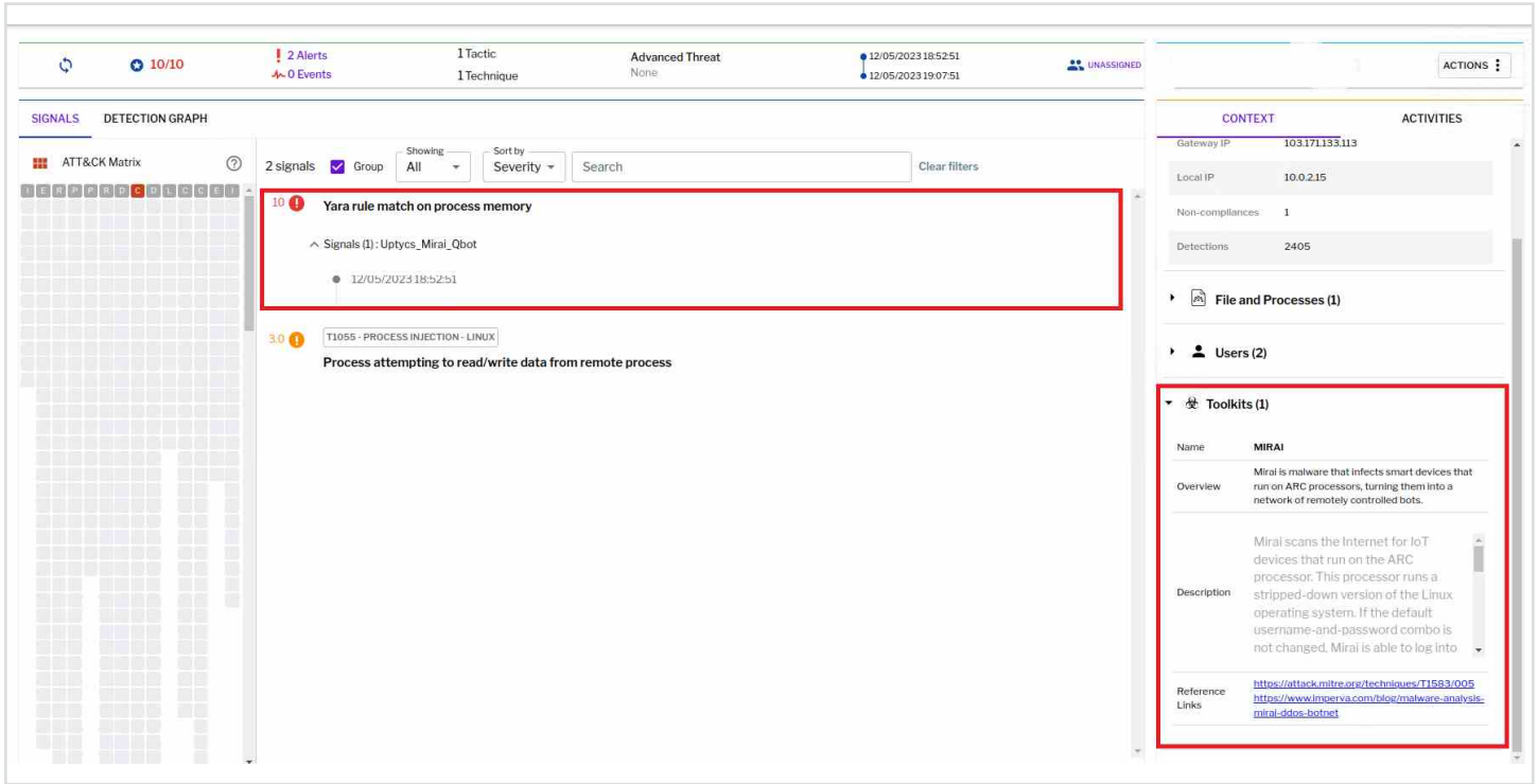
Figure 16–Uptycs XDR detection of Mirai malware
