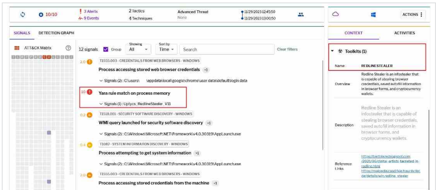
Figure 15–Uptycs XDR detection of Redline
