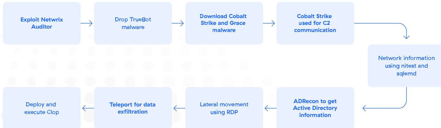
Figure 24: Clop attack chain
