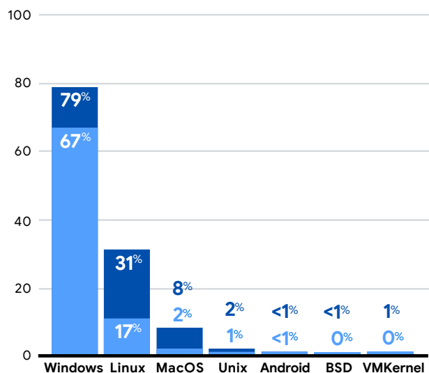
Operating System Effectiveness of Observed Malware Families, 2023
